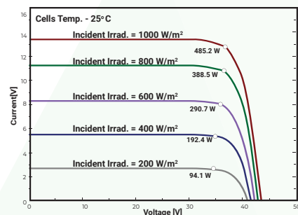
I-V Curve of 485 W at 25°C cell temp and different irradiance level
